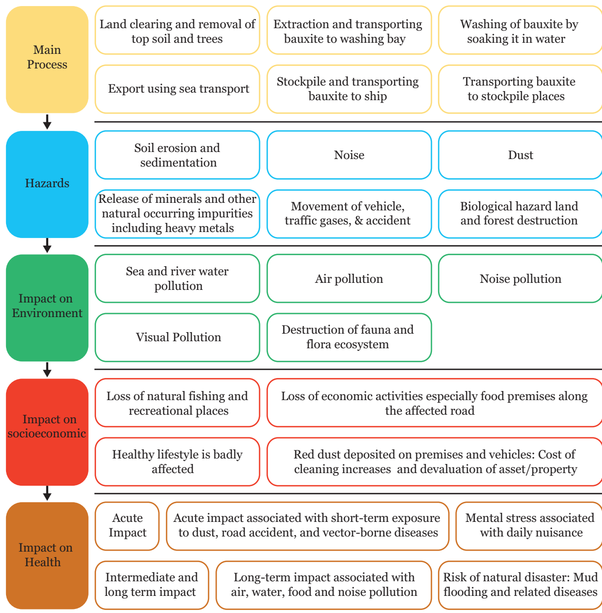
Figure 1: Linkages between bauxite mining activities and potentials impacts
