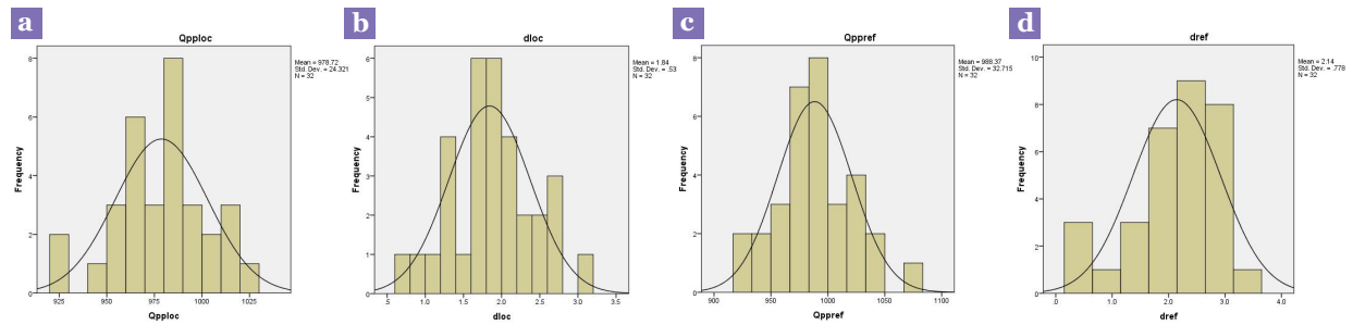
Figure 4: (a) The histogram of 32 dipole moment (Qpploc) for local phantom with mean 978.72 nAm, std dev. 24.32 nAm overlaid with normal distribution curve. (b) The histogram of 32 dipole difference in distance from nominal location (dlloc) for local phantom with mean 1.84 m, std dev. 0.53 m overlaid with normal distribution curve. (c) The histogram of 32 dipole moment (Qppref) for reference phantom with mean 988.38 nAm, std dev. 32.72 nAm overlaid with normal distribution curve. (d) The histogram of 32 dipole difference in distance from nominal location (dref) for reference phantom with mean 2.14 m, std dev. 0.78 m overlaid with normal distribution curve.
