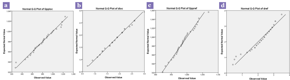
Figure 5: (a) The quantile-quantile (Q-Q) plot of 32 dipole moment (Qpploc) for local phantom overlaid with normal distribution line. (b) The quantile-quantile (Q-Q) plot of 32 dipole difference in distance from nominal location (dlloc) for local phantom overlaid with normal distribution line. (c) The quantile-quantile (Q-Q) plot of 32 dipole moment (Qppref) for reference phantom overlaid with normal distribution line. (d) The quantile-quantile (Q-Q) plot of 32 dipole difference in distance from nominal location (dref) for reference phantom overlaid with normal distribution line.
