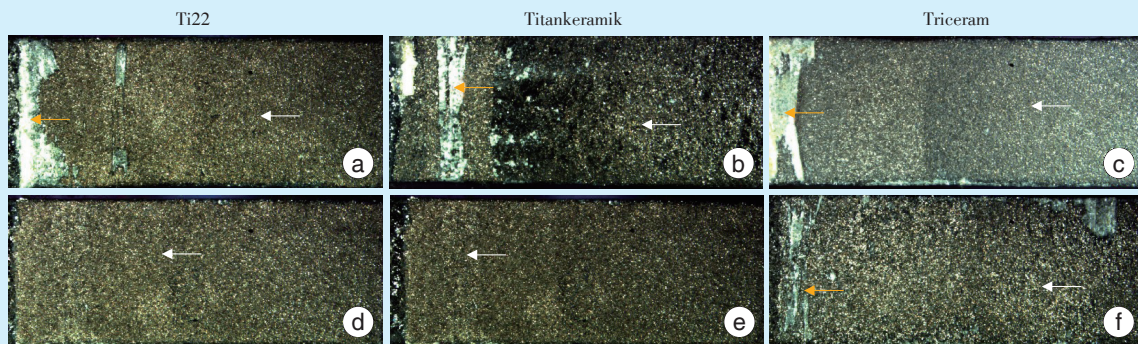
Figure 5 Typical fracture modes of the three types of porcelain
