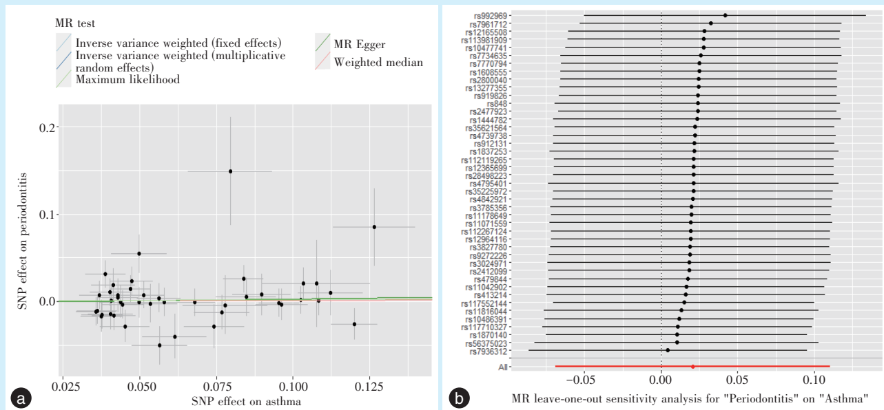
a: scatter plots of the MR analysis. Black dots denote the genetic instruments used in the primary MR analysis. The slope of each line corresponds to the estimated MR effect in different models. b: leave-one-out analysis. Each black point represents the IVW MR method applied to estimate the causal effect of periodontitis on asthma, excluding that particular variant from the analysis. The red point represents the IVW estimate using all SNPs. MR: Mendelian randomization; IVW: inverse variance weighted
