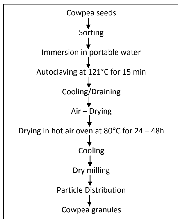
Figure 1: Flow diagram for production of Cowpea granules (carrier).
