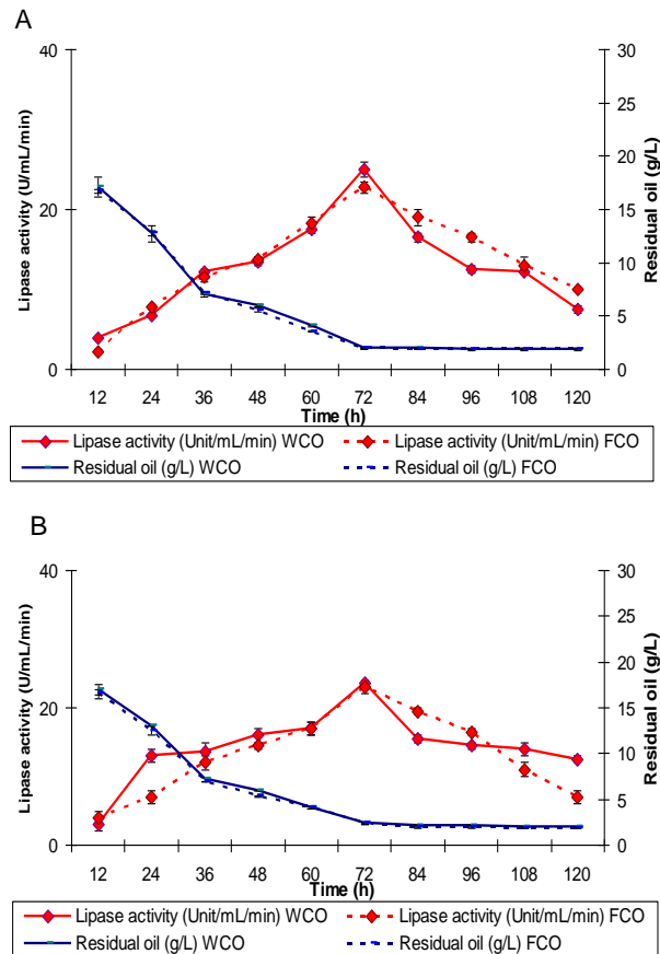
Figure 5: Lipase activity and residual oil content associated with P(3HB) biosynthesis by using FCO or WCO as the sole carbon sources. A) C. necator H16 B) C. necator PHB - 4/pBBREE32d13. Oil concentration and urea concentration were 20.0 g/L and 1.08 g/L respectively. Samples were incubated for 72 h, at 30 °C, initial pH 7.0, and shaken at 200 rpm.
