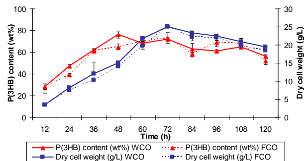
Figure 3: Time profile of P(3HB) biosynthesis by C. necator H16, using WCO or FCO as the sole carbon sources.
