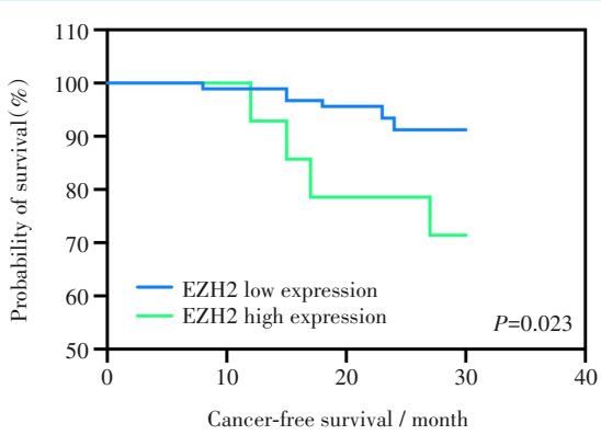
Figure 3 Kaplan-Meier survival curve of cancer-free survival in OLK patients with high and low EZH2 expression
