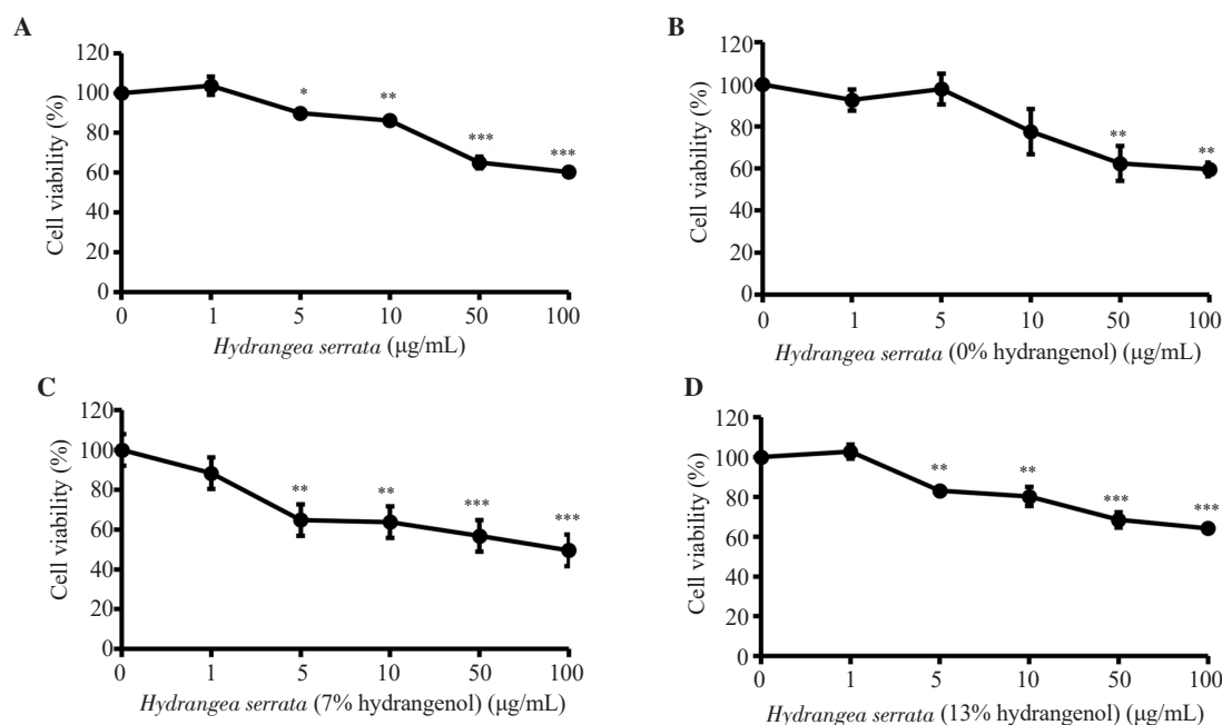
Figure 1. Effect of Hydrangea serrata ( H. serrata ) extracts on the viability of HepG2 cells with or without hydrangenol, a key indicator component. (A) Natural H. serrata extract without controlled hydrangenol concentration, and with (B) 0%, (C) 7%, (D) 13% hydrangenol. Cell viability was determined by MTT assay after 24 hours of treatment with the indicated concentration. Relative cell viability of 0 \mu\text{g}/\text{mL} control was set as 100%. Data are presented as mean \pm SD and analyzed by ANOVA. Each experiment was performed in duplicate and repeated at least three times. * P < 0.05 , ** P < 0.01 , *** P < 0.001 compared with the control.
