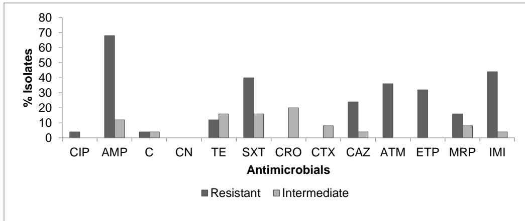
Figure 1: Percentage (%) E. coli isolates from Tilapia with resistant or intermediate responses to the test antimicrobials. AMP-ampicillin; CTX-cefotaxime; ATM-aztreonam; ETP-ertapenem; C-chloramphenicol; IMI-imipenem; CAZ-ceftazidime; MRP-meropenem; CIP-ciprofloxacin; SXT-sulfamethoxazole trimethoprim; CN-gentamicin; TE-tetracycline; CRO-ceftriaxone
